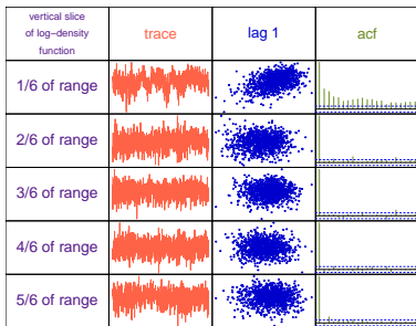
Figure 14: The chains of the log-density estimates at five equally-spaced vertical slices for the slice sampling-based Bayesian density estimation displayed in Figure 13.
