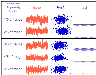
Figure 6: The chains corresponding to the density estimate object densLongerChains with a warm-up of size 2,000, kept samples of size 3,500 and a thinning factor of 5.
