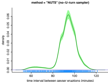
Figure 3: Bayesian density estimate for the data from Figure 1 using the no-U-turn sampler. The pale green shaded region corresponds to approximate 95% pointwise credible intervals. The data are shown as tick marks, with some jittering, at the base of the plot.
