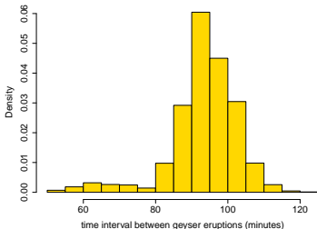
Figure 1: A probability histogram for the time intervals (minutes) between all 3,507 adjacent pairs of eruptions of the Old Faithful Geyser during the year 2011. The histogram bins correspond to the default call to the R function hist() .
